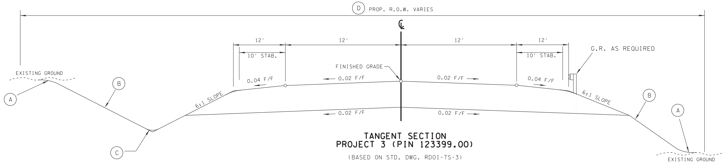
SECTION E-E
