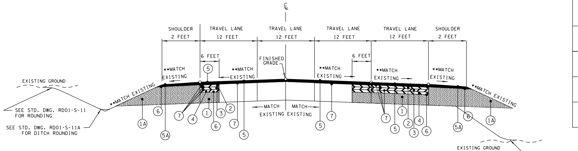
TANGENT SECTION STATE ROUTE 247 FROM THE PROPOSED INTERSECTION WITH CLEBURNE ROAD AND EXTENDING TO APPROXIMATELY 400 FEET WEST (BASED ON STD. DWG. RD01-TS-7)
