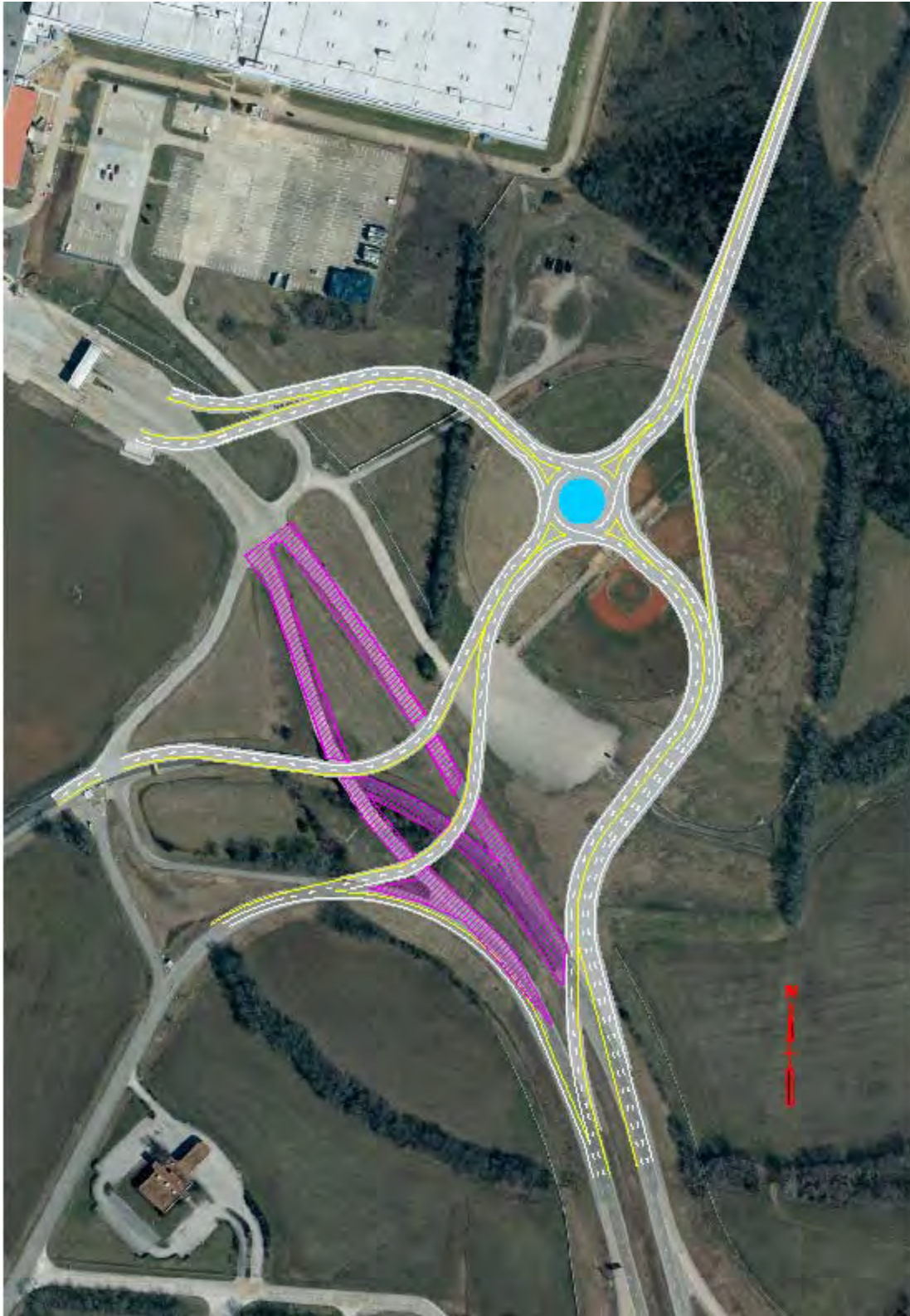
Figure 7: Roundabout
