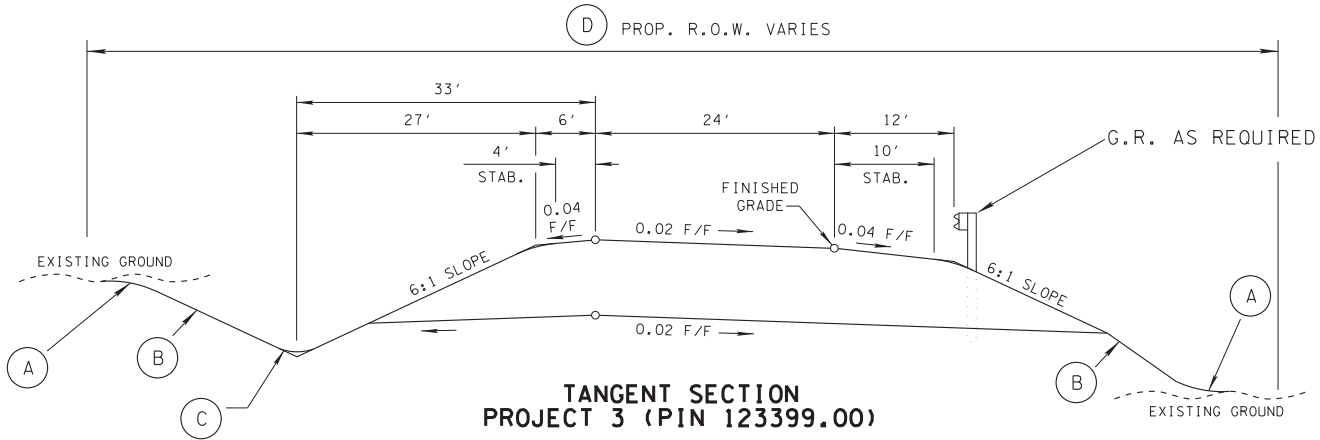
SECTION G-G
