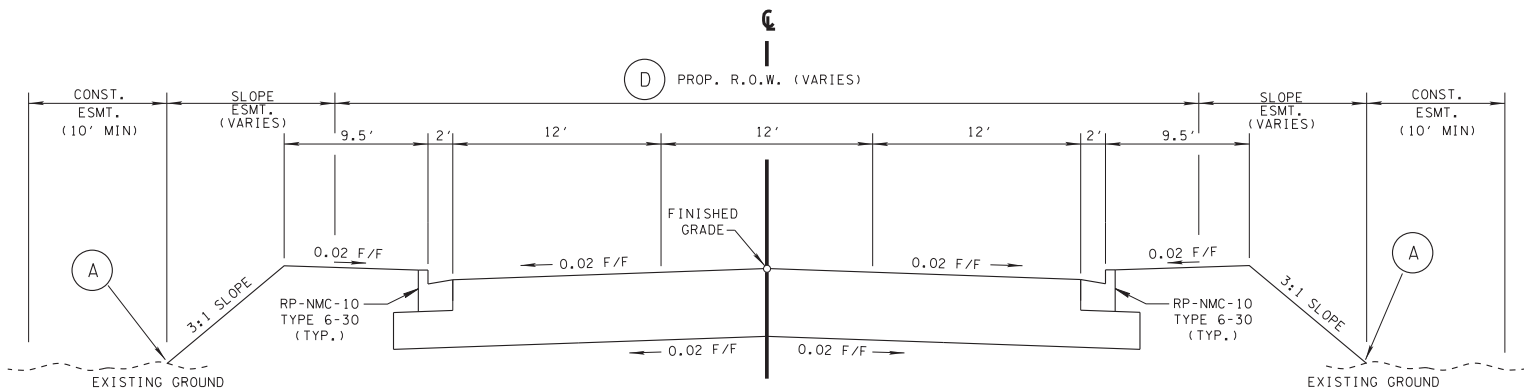
TANGENT SECTION PROJECT 1 (PIN 117319.01) (BASED ON STD. DWG. RD01-TS-6A) S.R. 247 (BEECHCROFT RD.) STA. 18+45.00 TO STA. 21+55.00
