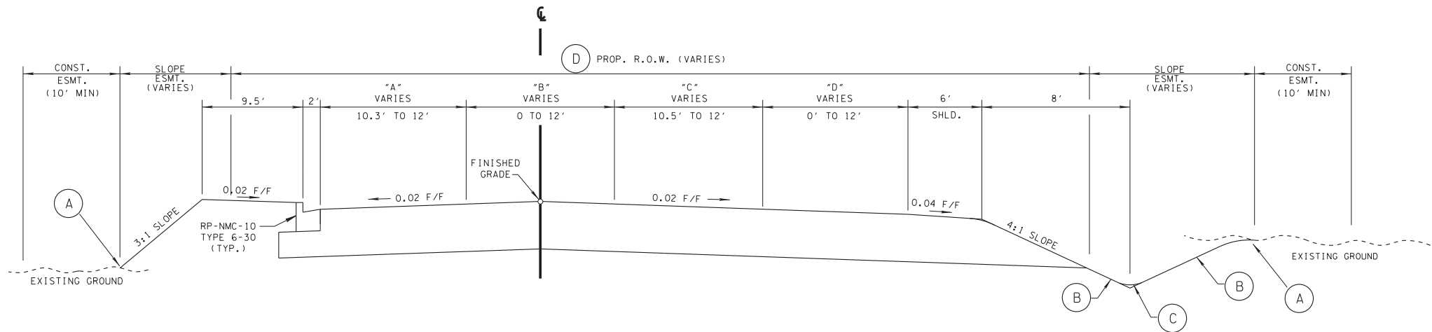
TANGENT SECTION PROJECT 1 (PIN 117319.01) (BASED ON STD. DWG. RD01-TS-2) S.R. 247 (BEECHCROFT RD.) STA. 12+25.00 TO STA. 17+64.00
