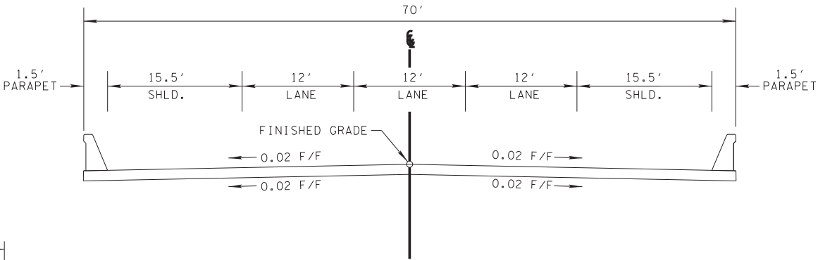
TANGENT BRIDGE SECTION PROJECT 3 (PIN 123399.00) SECTION B-B BRIDGE TO ACCOMMODATE FUTURE 5-LANE SECTION (5-11' LANES WITH 6' SHOULDERS)
