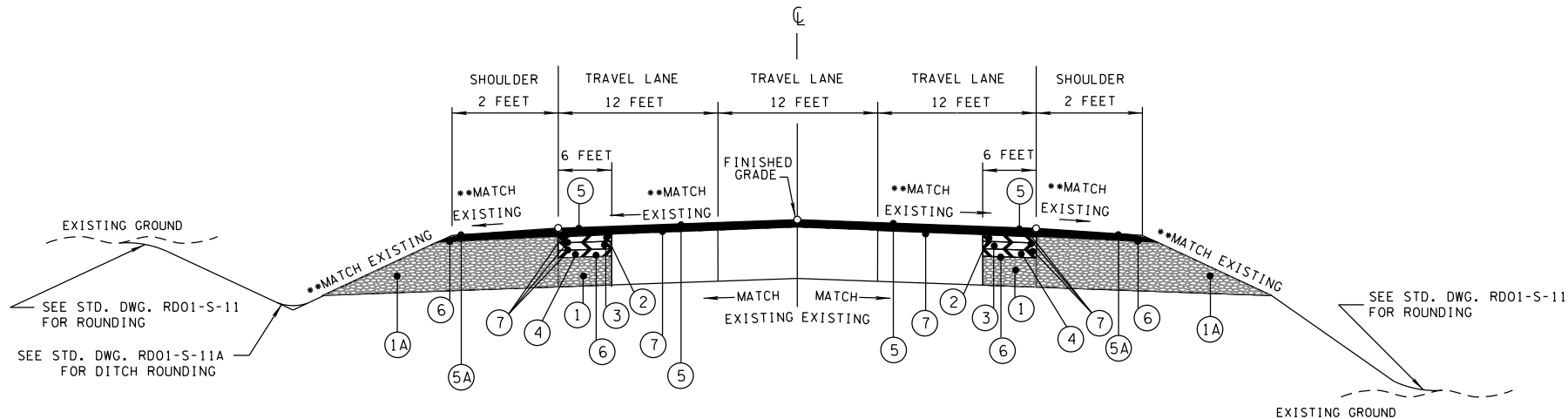
TANGENT SECTION STATE ROUTE 247 FROM THE PROPOSED INTERSECTION WITH CLEBURNE ROAD AND EXTENDING TO APPROXIMATELY 500 FEET EAST & CLEBURNE ROAD FROM THE PROPOSED INTERSECTION WITH STATE ROUTE 247 AND EXTENDING TO APPROXIMATELY 300 FEET SOUTH (BASED ON STD. DWG. RD01-TS-7)
